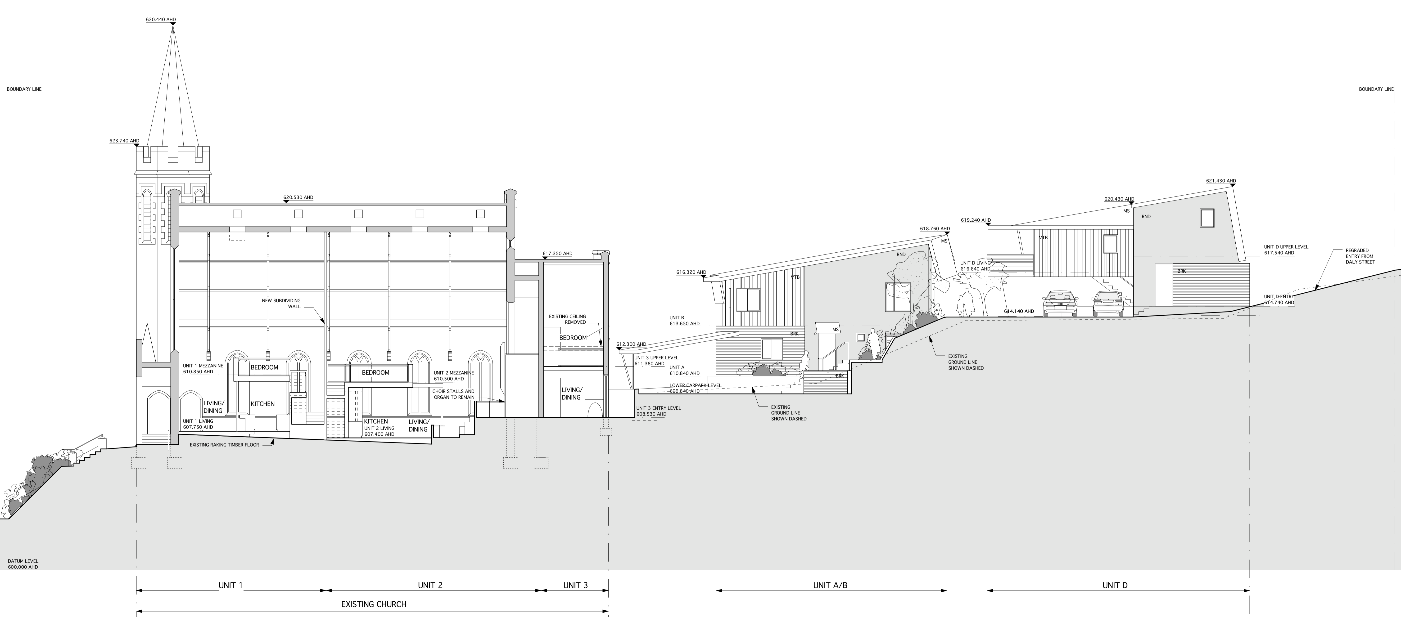
SECTION AA 1:100
